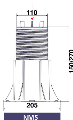
Figure 2 Typical "New-Maxi NM5" specimen.
